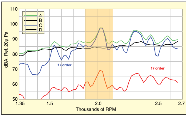
Figure 9. Engine second-order data example.
